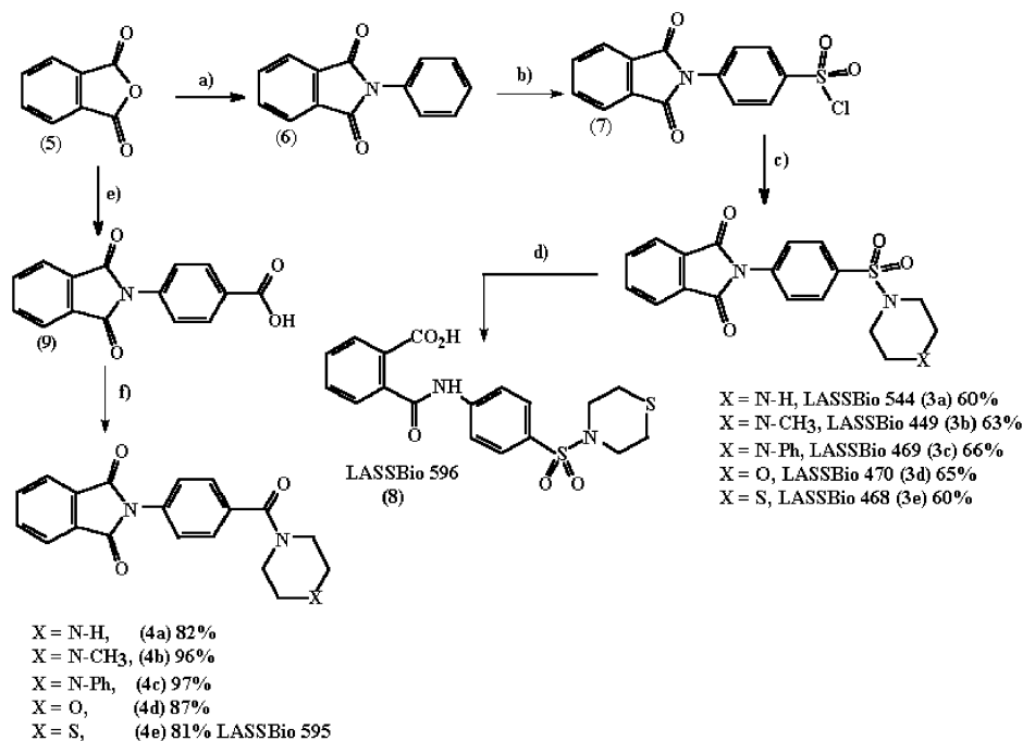
Scheme 1. (a) C 6 H 5 NH 2 , reflux, 1 h; 86%; (b) ClSO 3 H, PCl 5 , 50 °C, 30 min, 70%; (c) functionalized piperazines, CH 2 Cl 2 , rt, 30 min, 60–66%; (d) LiOH, THF, MeOH, H 2 O, rt, 10 min, 77%; (e) 4-CO 2 HC 6 H 4 NH 2 , AcOH, reflux, 1 h, 91%; (f) (1) SO 2 Cl, DMF (cat), reflux, 1 h; (2) CH 2 Cl 2 , functionalized piperazines, rt, 30 min, 81–97%.
